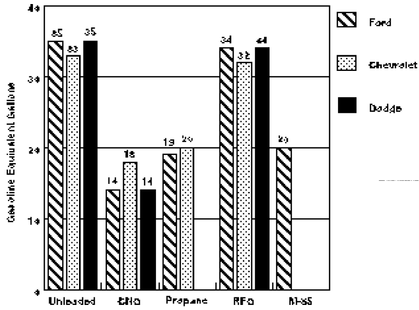
Figure 6. Energy Supply on CleanFleet Vans
