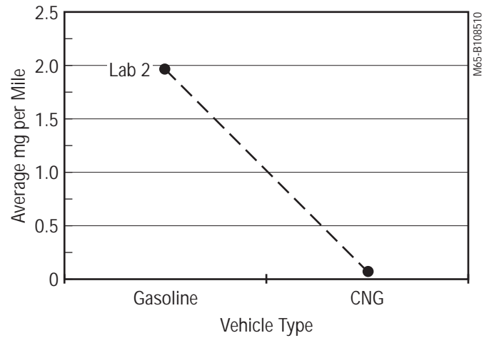
Figure 11. Comparison of C 6 H 6 from the two types of vehicles
