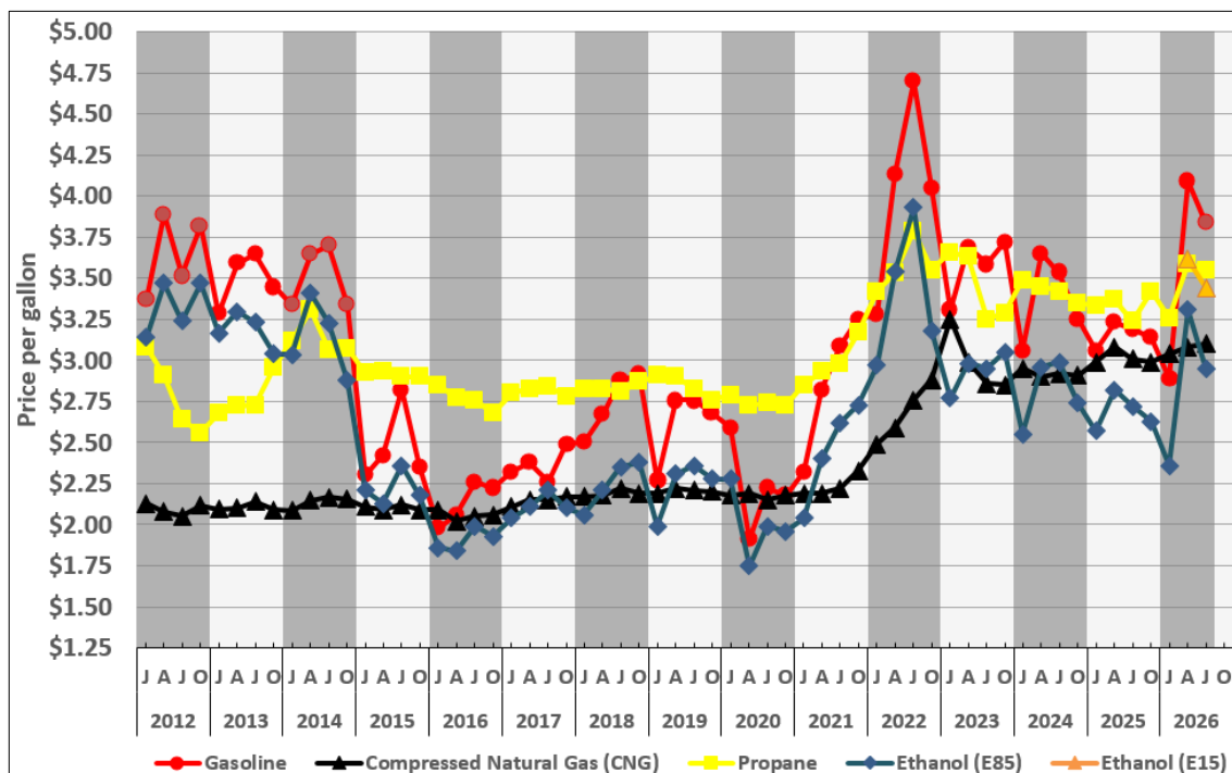
FIGURE 20 ALTERNATIVE FUEL PRICES VERSUS GASOLINE
