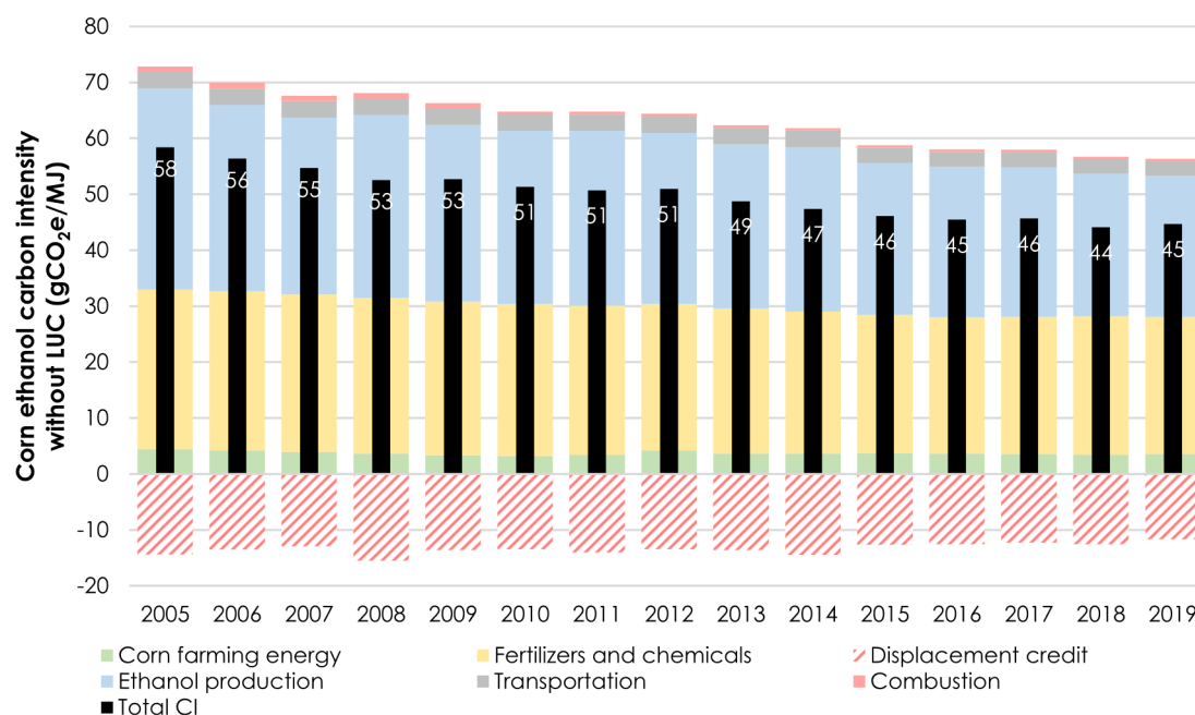
Figure 4. Carbon intensity ( \text{gCO}_2\text{e/MJ} undenatured ethanol) of corn ethanol without LUC for 2005–2019.
